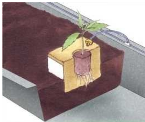
This cutaway drawing shows how nutrient delivery is simple and easy with a top-feed bat system. Aerated nutrient solution is metered via
