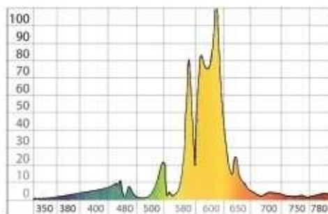
Color spectrum of Spectrum HPS Super bulb
