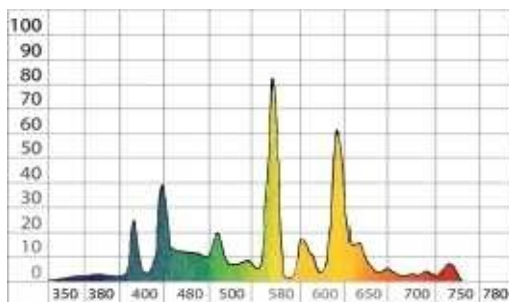
Light spectrum of Warm White (2700 K) fluorescent bulb
