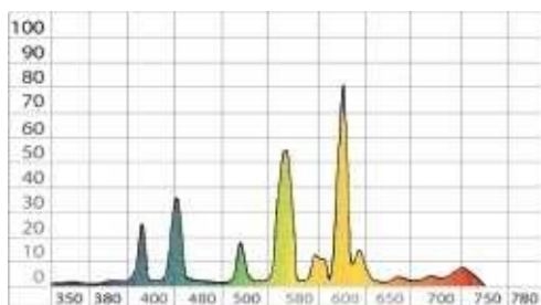
Light spectrum of Warm White (2700 K) fluorescent bulb
