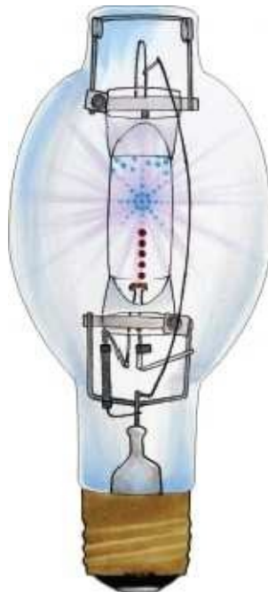
Metal Halide bulb showing reaction.
