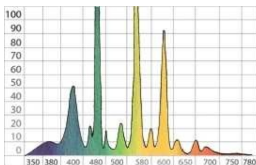
Color spectrum of Cool Deluxe Sunmaster bulb
