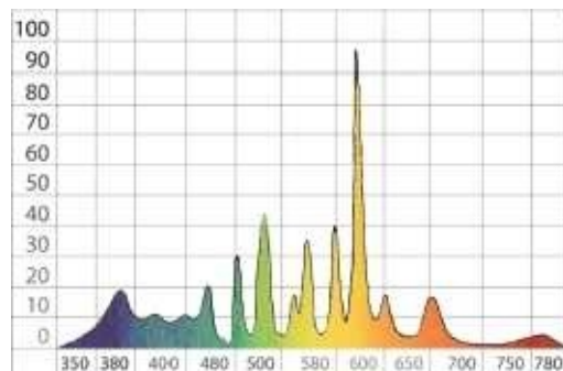
Color spectrum of Warm Deluxe Sunmaster bulb
